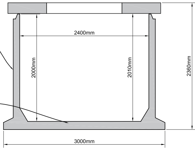
TANK PLAN
