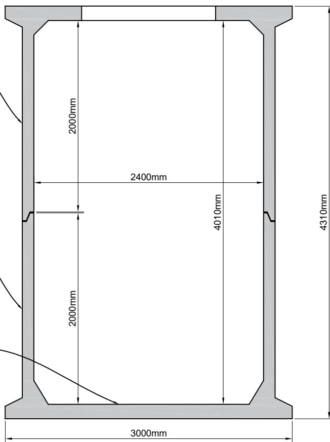
TANK PLAN
