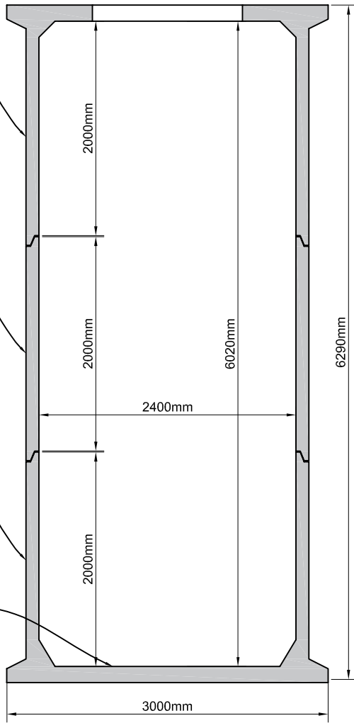
TANK PLAN
